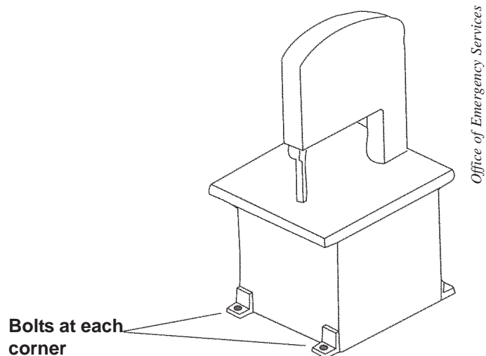
Figure 51—Bolting equipment. Light equipment can be bolted to a concrete floor with expansion bolts. For methods of securing heavier equipment, consult an engineer.
